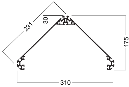
[Sectional view]
