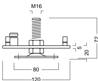
Adjustable foot
